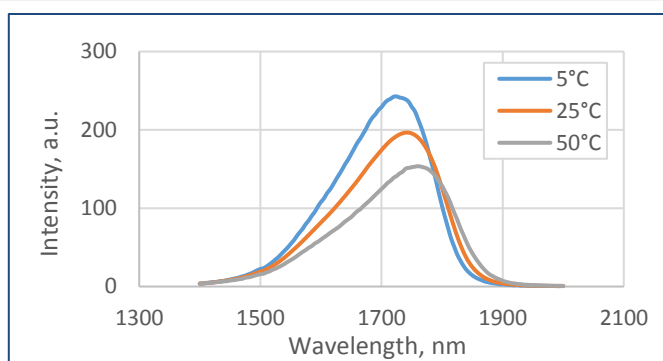
Spectra at different temperatures (qCW 3 , 25 mA)
