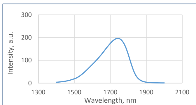
Typical spectrum (qCW 3 , 25 mA)
