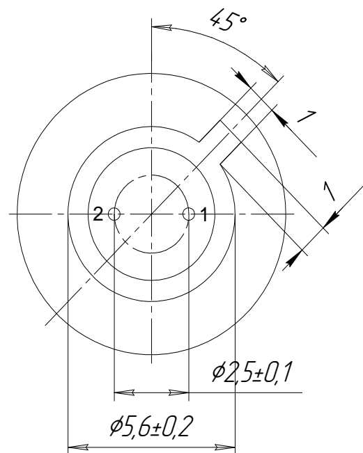
BOTTOM VIEW
