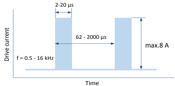
Pulse mode
