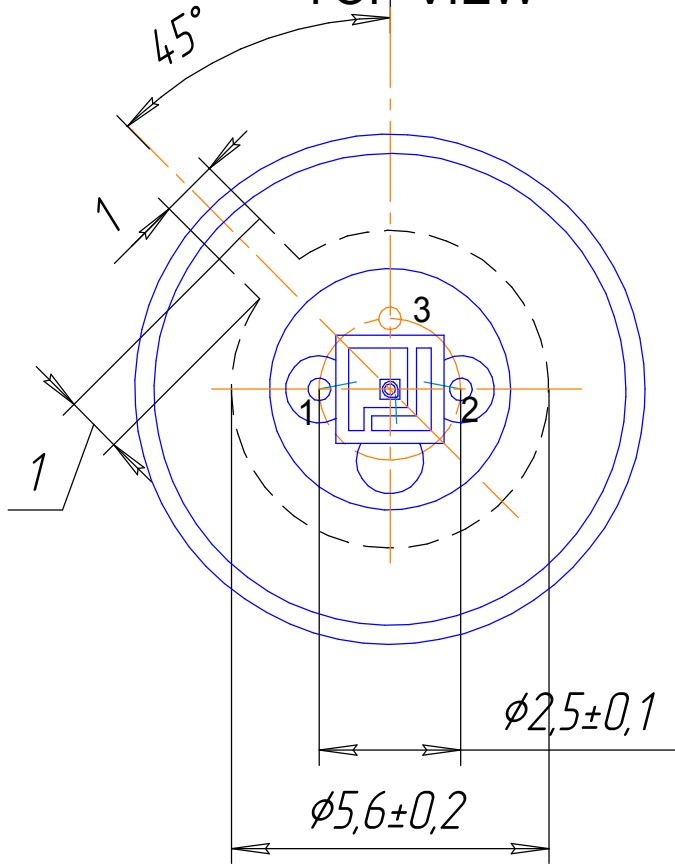
TOP VIEW
